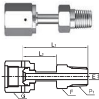
Welded Male Connector (PT) (TWMCR)
