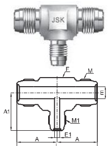
Reducing Union Tee (TUT)
