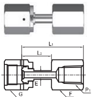
Welded Female Connector (NPT) (TWFCN)
