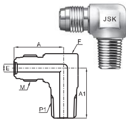
Male Elbow (PT) (TMER)
