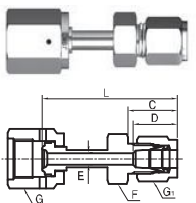
Welded Lok Connector (TWLC)
