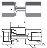
Welded Female Connector (PT) (TWFCR)
