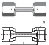
Welded Female Union (TWFU)
