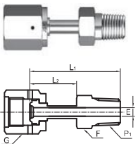
Welded Male Connector (NPT) (TWMCN)
